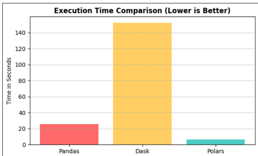
Figure 6.1 Libraries comparison of execution time
