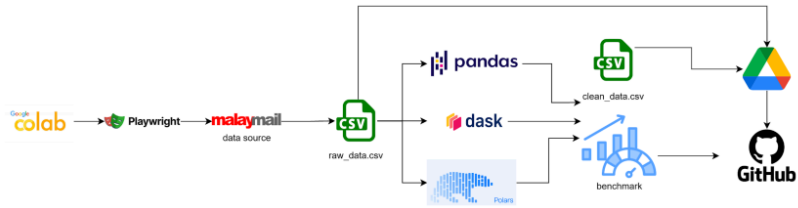
Diagram 2.2 Tools and Frameworks Used
