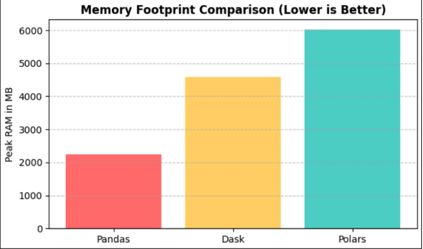
Figure 6.2 Libraries comparison of memories footprint
